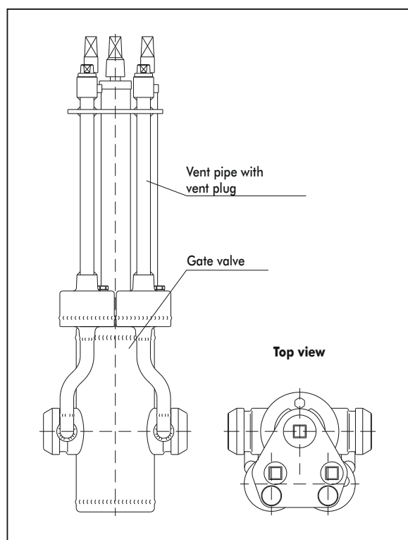
Picture 6 ASR with bottom arranged rotary gate valve
